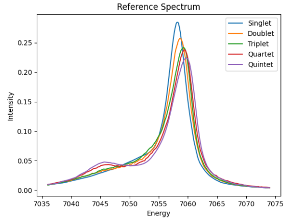
Figure 7: The reference spectra plotted with provided data for different spin states.
