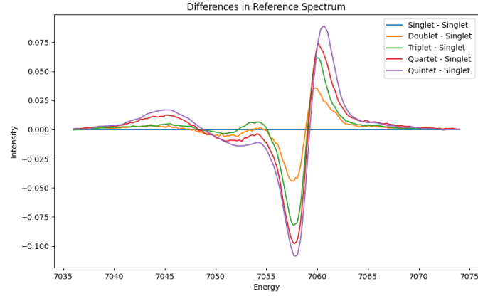
Figure 8: The reference difference spectra with transient signals plotted with provided data for different transitions.
